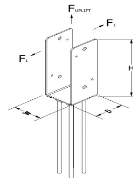
Loading Directions
